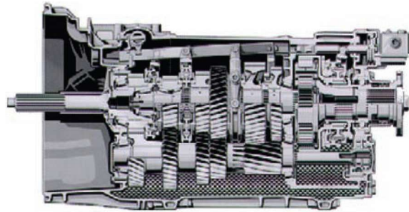
Daimler Chrysler 16 speed G240-16
